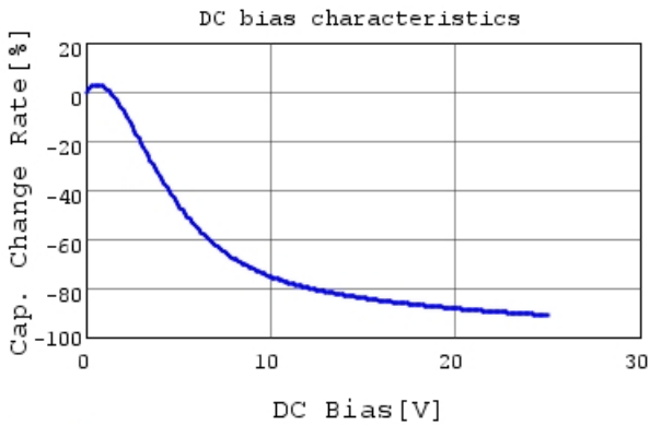
GRM188R61E225MA12 C-DC bias capchange, 25.0c
