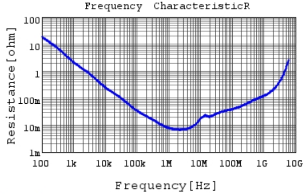
GRM188R61E225MA12 R DCOV,25degC
