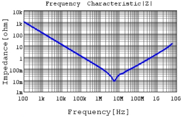
GRM188R61E225MA12 |Z| DCOV,25degC
