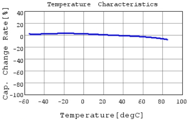
GRM188R61E225MA12 C-Temp. capchange, DCO.OV,
