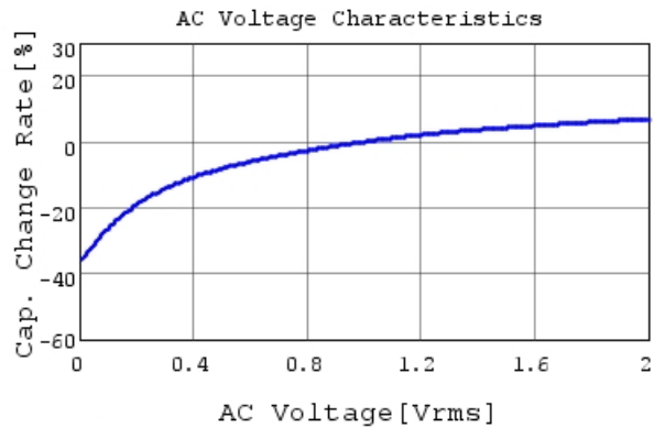
GRM188R61E225MA12 C-AC Voltage capchange, Dc
