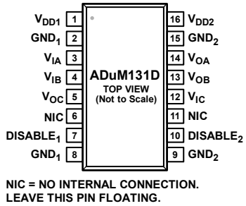
Figure 9. ADuM131D Pin Configuration
