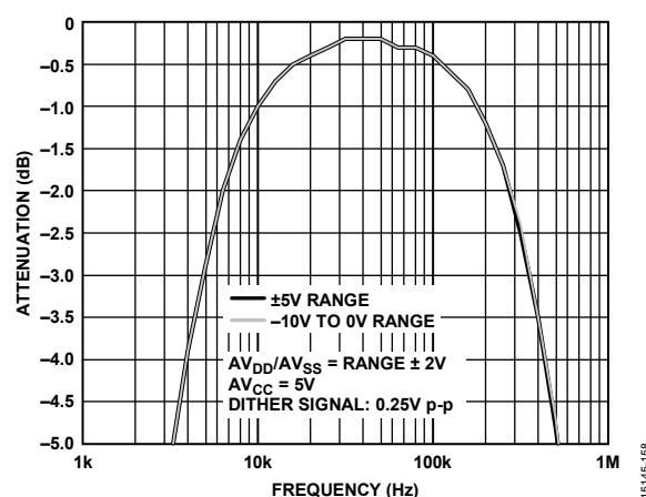
Figure 62. Dither Input to DAC Output Attenuation vs. Frequency ( \pm 5 V Range and -10 V to 0 V Range)
