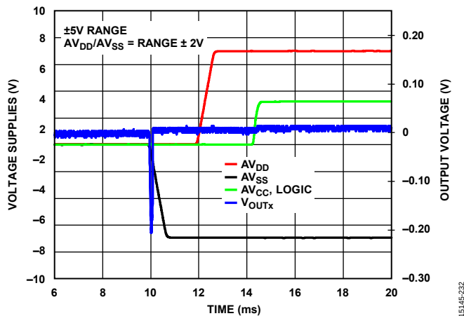
Figure 32. Power-Up Glitch
