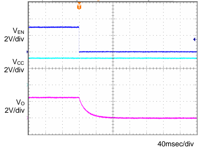
Fig.18 OFF sequence 2 Co=1µF, Ta=-40°C
