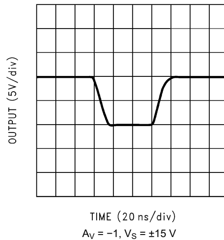
Figure 5-80. Large-Signal Pulse Response
