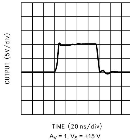
Figure 5-82. Large-Signal Pulse Response
