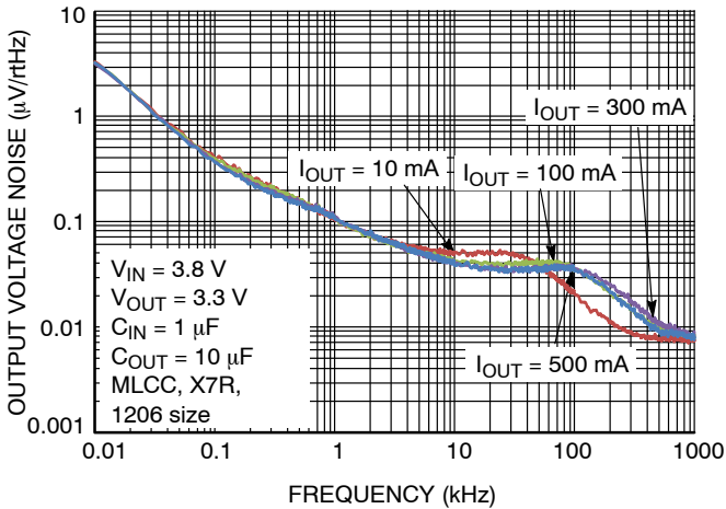
Figure 6. Output Voltage Noise Spectral Density for V_{\text{OUT}} = 3.3 \text{ V} , C_{\text{OUT}} = 10 \mu\text{F}
