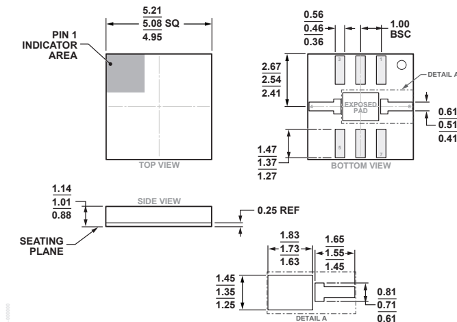
8-Terminal Chip Array Small Outline No Lead Cavity [LGA_CAV] 5.08 mm × 5.08 mm Body and 1.01 mm Package Height (CE-8-1)
