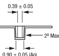
Figure 8. SC-79 Tape and Reel Dimensions
