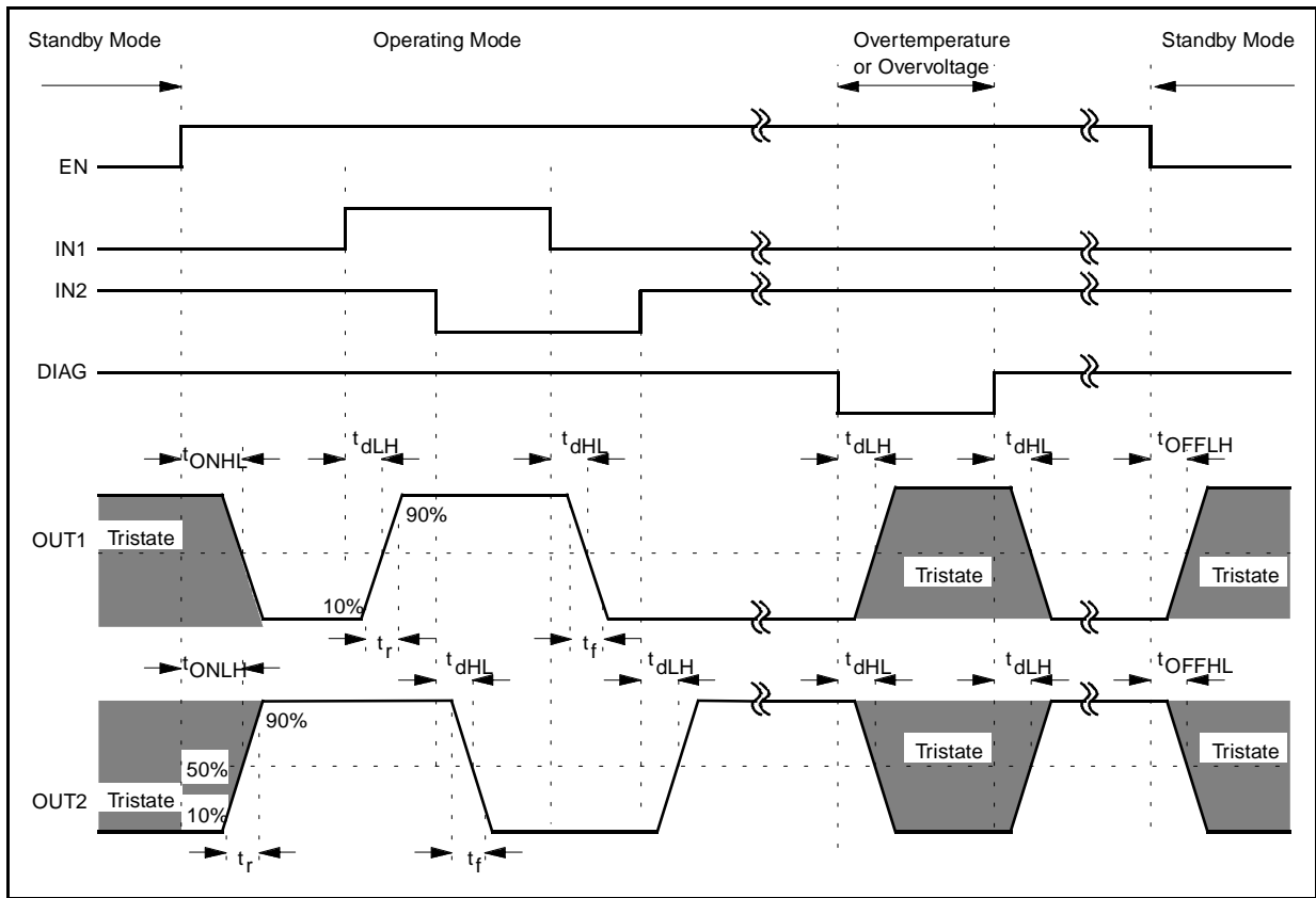
Figure 2. Timing Diagram.
