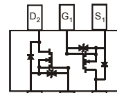
Equivalent Circuit
