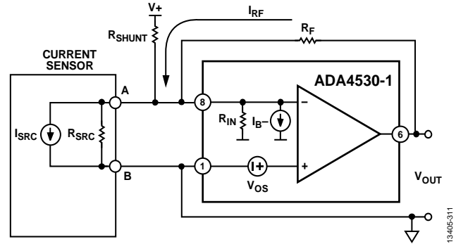
Figure 106. TIA Circuit
