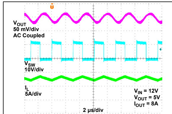
FIGURE 2-48: Switching Waveforms ( V_{OUT} = 5V , I_{OUT} = 8A ).
