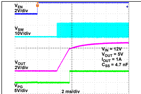
FIGURE 2-45: 2.5 ms Soft-Start Time.
