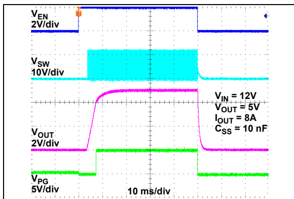
FIGURE 2-44: Enable Turn-On/Turn-Off.
