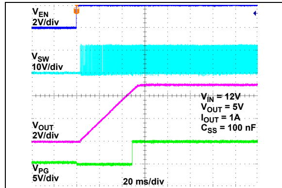
FIGURE 2-46: 40 ms Soft-Start Time.
