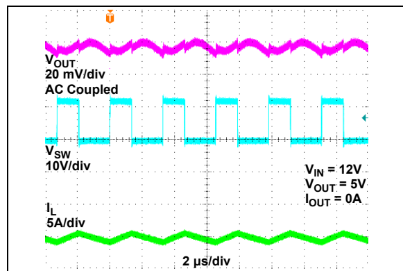
FIGURE 2-47: Switching Waveforms ( V_{OUT} = 5V , I_{OUT} = 0A ).
