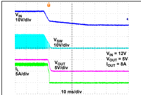
FIGURE 2-43: V_{IN} Soft Turn-Off.
