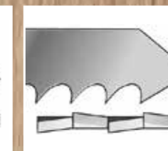
INCLINED SHARPENED, CROSSED TEETH For fast cuts in hardwood and softwood.
