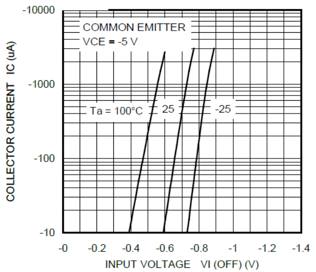
Fig. 10.6 RN2314 I_C - V_{I(OFF)}
