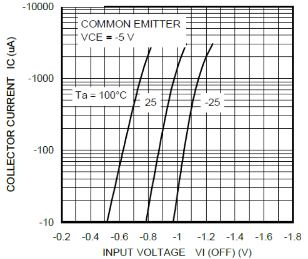
Fig. 10.8 RN2316 I_C - V_{I(OFF)}
