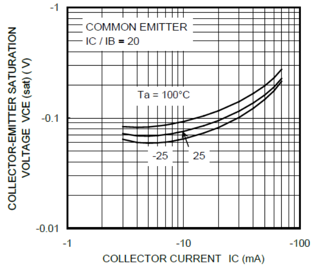
Fig. 10.20 RN2318 V_{CE(sat)}-I_C
