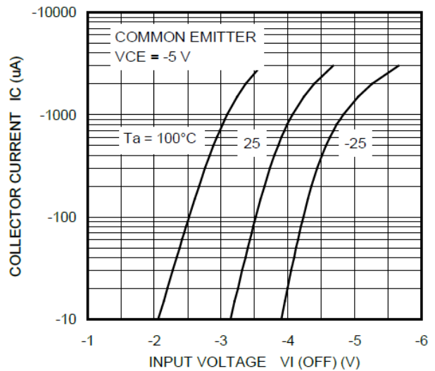
Fig. 10.10 RN2318 I_C - V_{I(OFF)}
