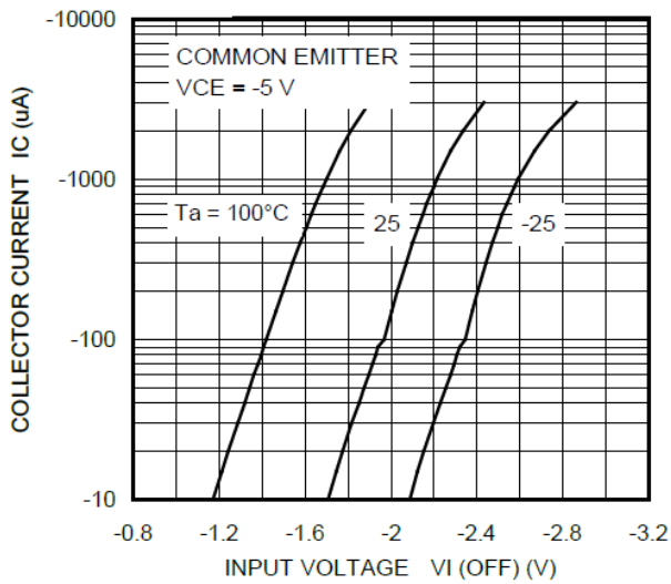
Fig. 10.9 RN2317 I_C - V_{I(OFF)}
