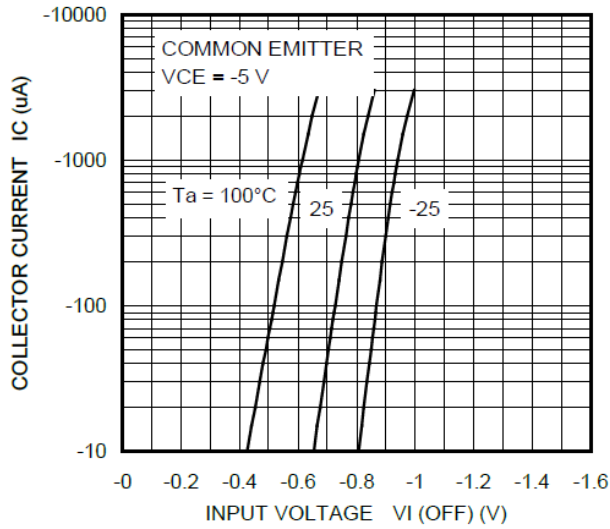
Fig. 10.7 RN2315 I_C - V_{I(OFF)}
