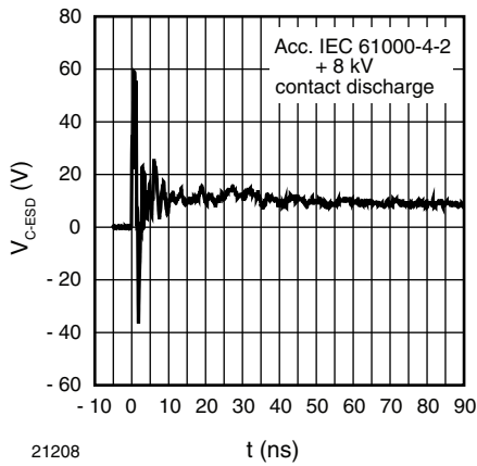
Fig. 7 - Typical Clamping Performance at + 8 kV Contact Discharge (acc. IEC 61000-4-2)
