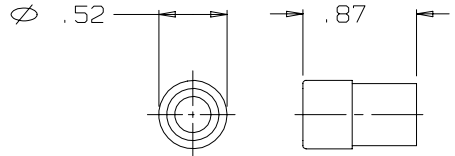
AP-107-27 CABLE SEAL ASSEMBLY (1 REQ'D)
