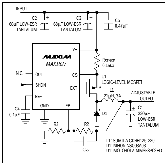
Figure 8. MAX1627 Typical Operating Circuit
