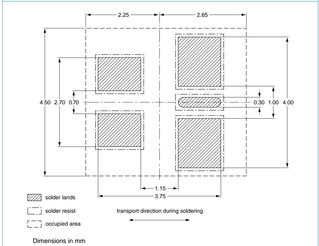
Fig 15. Wave soldering footprint PESDxL4UG (SOT353/SC-88A)
