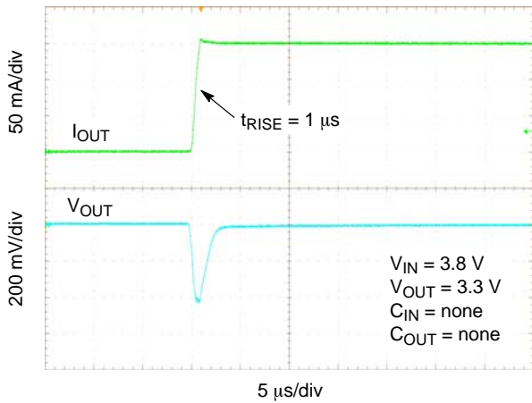
Figure 34. Load Transient Response – 1 \text{ mA} to 150 \text{ mA} – C_{OUT} = \text{None}
