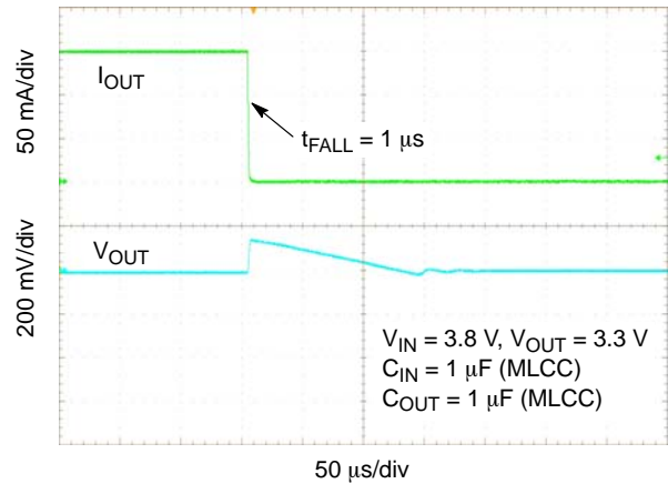
Figure 37. Load Transient Response – 150 \text{ mA} to 1 \text{ mA} – C_{OUT} = 1 \mu\text{F}
