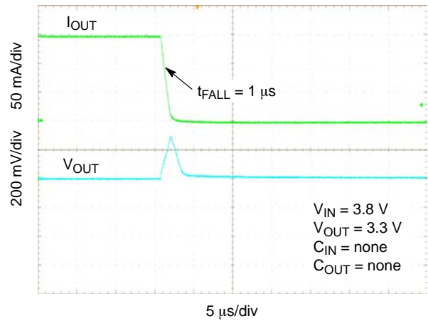
Figure 35. Load Transient Response – 150 \text{ mA} to 1 \text{ mA} – C_{OUT} = \text{None}
