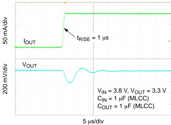
Figure 36. Load Transient Response – 1 \text{ mA} to 150 \text{ mA} – C_{OUT} = 1 \mu\text{F}
