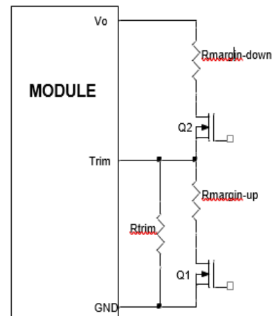
Figure 51. Circuit Configuration for margining Output voltage.
