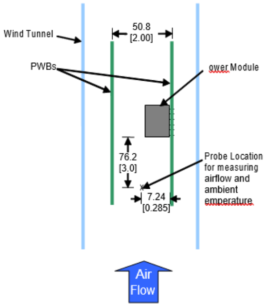
Figure 53. Thermal Test Setup.
