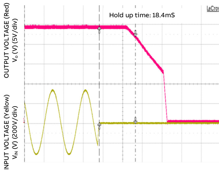
Figure 7. Typical Hold-up Waveforms ( V_{IN} = 230\text{V} , 100% Load)
