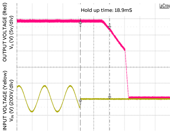
Figure 6. Typical Hold-up Waveforms ( V_{IN} = 115\text{Vac} , 100% Load)
