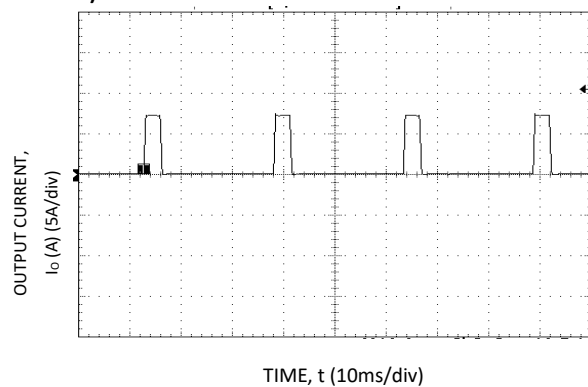
Figure 18. Output short circuit Current ( V_{IN} = 5.0Vdc , V_o = 0.75Vdc ).
