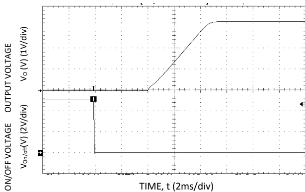
Figure 15. Typical Start-Up Using Remote On/Off with Low-ESR external capacitors (7x150uF Polymer) ( V_{IN} = 5.0Vdc , V_o = 3.3Vdc , I_o = 3A , C_o = 1050\mu F ).
