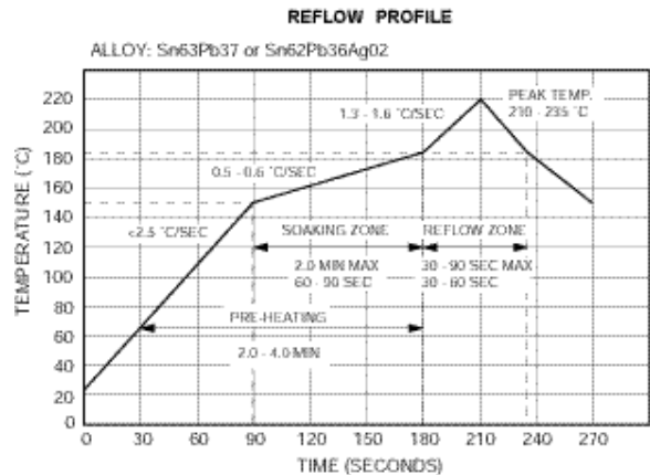
Figure 35. Reflow Profile.
