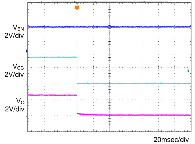
Figure 14. OFF sequence 1 C_o=1\mu F, T_a=105^\circ C
