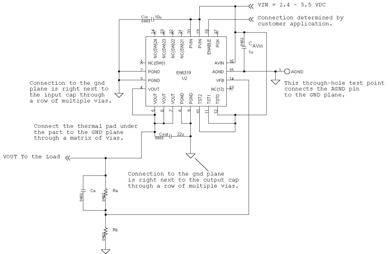
Figure 7. Engineering Schematic with Critical Components
