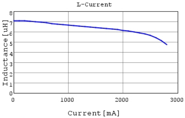
LQH5BPN6R8NT0 L-Current 20degC
