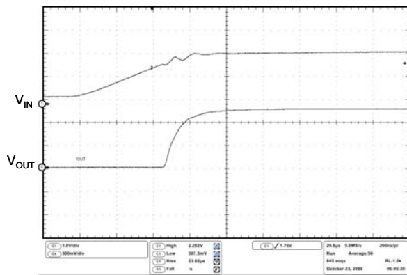
Figure 30. Start transient
