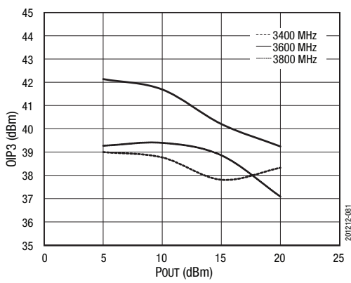
Figure 81. OIP3 vs Pout
