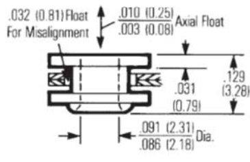
Rear panel mounting
