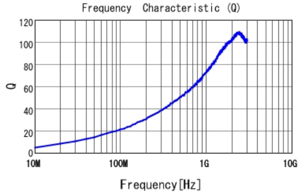
LQW2BAS6N8J00 Q
