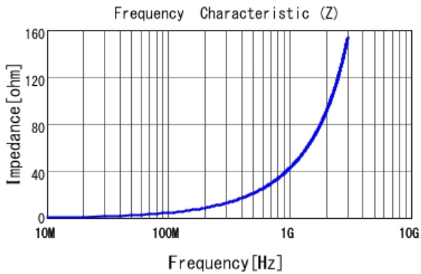
LQW2BAS6N8J00 |Z|
