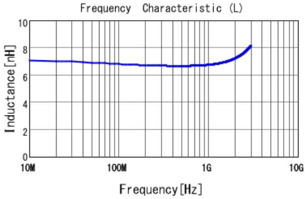
LQW2BAS6N8J00 L
