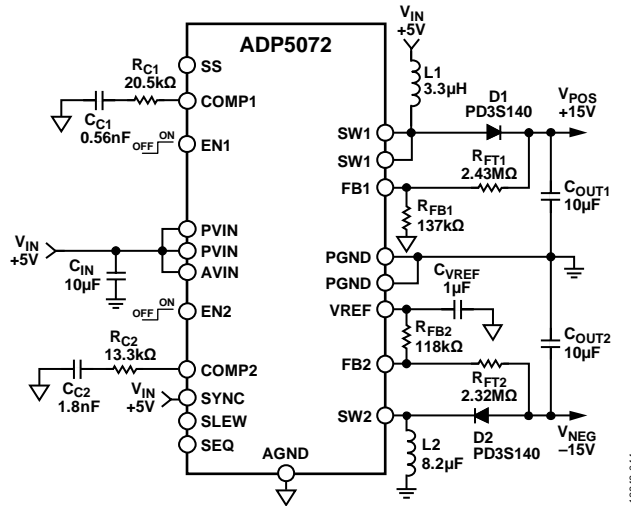
Figure 46. Typical +5 V to ±15 V Application
