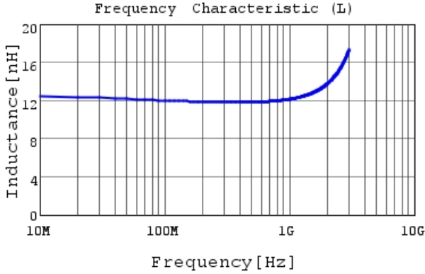
LQW2BAS12NJ00 L
