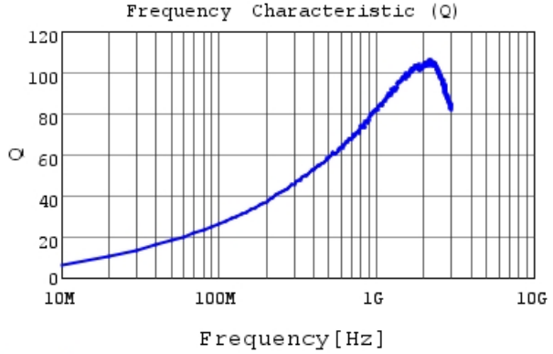
LQW2BAS12NJ00 Q
