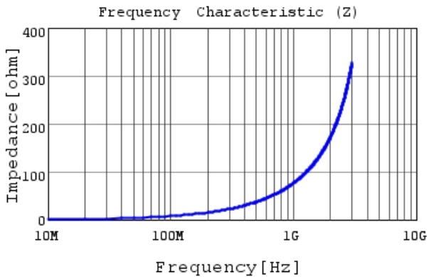
LQW2BAS12NJ00 |Z|
