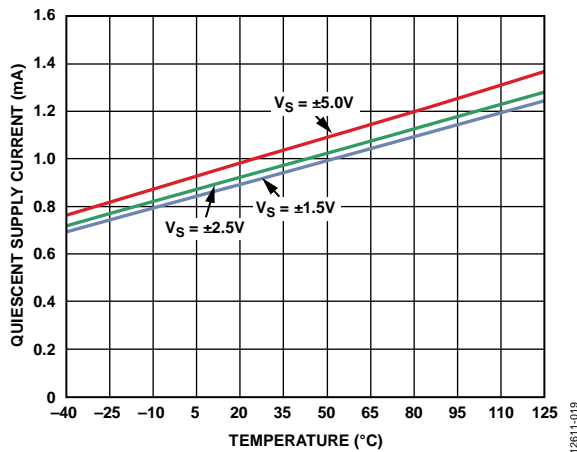
Figure 24. Quiescent Supply Current vs. Temperature
