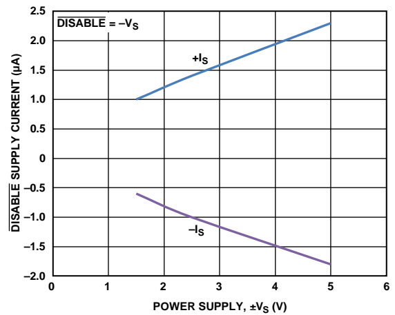
Figure 27. \overline{\text{DISABLE}} Supply Current vs. Power Supply, \pm V_S
