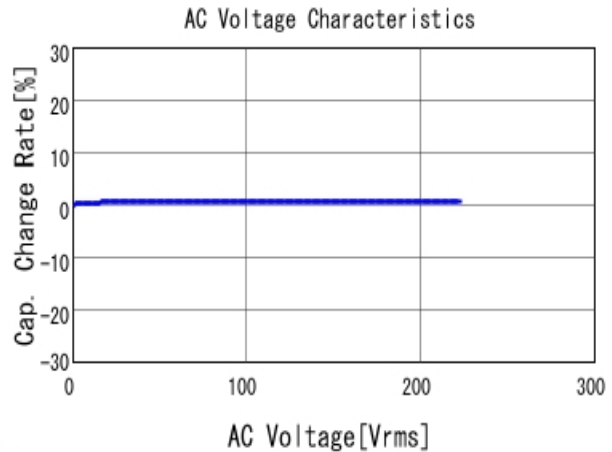
■ GRM31A7U2J102JW31 C-AC Voltage capchange, DCOV, 25.0d
