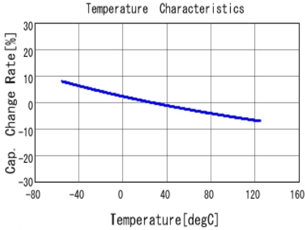
■ GRM31A7U2J102JW31 C-Temp. capchange, DCOV, AC1Vrms
