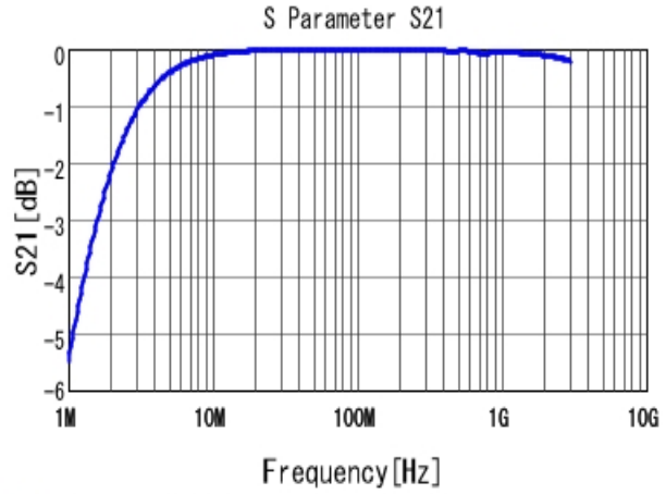
■ GRM31A7U2J102JW31 S21 DCOV, 25degC
