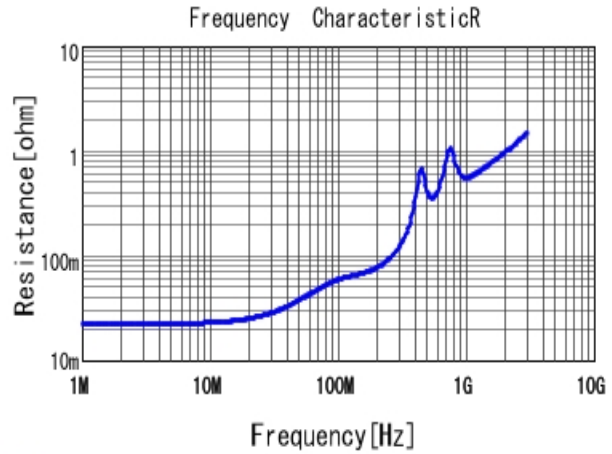
■ GRM31A7U2J102JW31 R DCOV, 25degC
