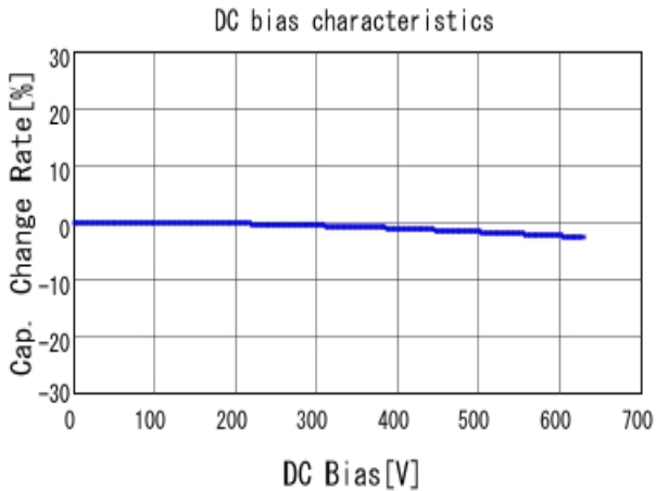
■ GRM31A7U2J102JW31 C-DC bias capchange, 25.0degC, AC1V
