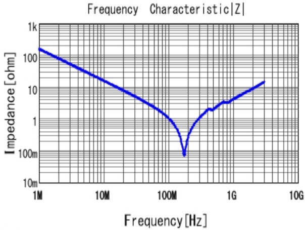
■ GRM31A7U2J102JW31 |Z| DCOV, 25degC
