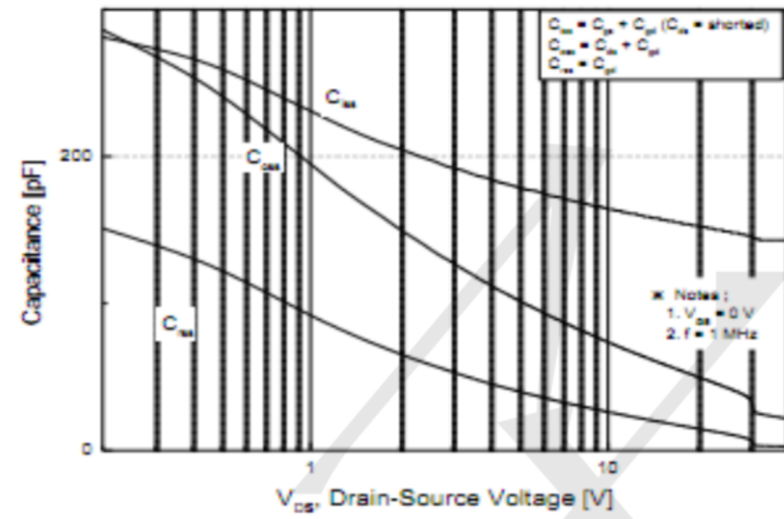
Fig.8 Capacitance Characteristics
