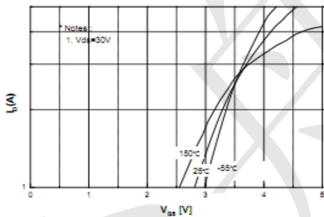
Fig.5 Transfer Characteristics
