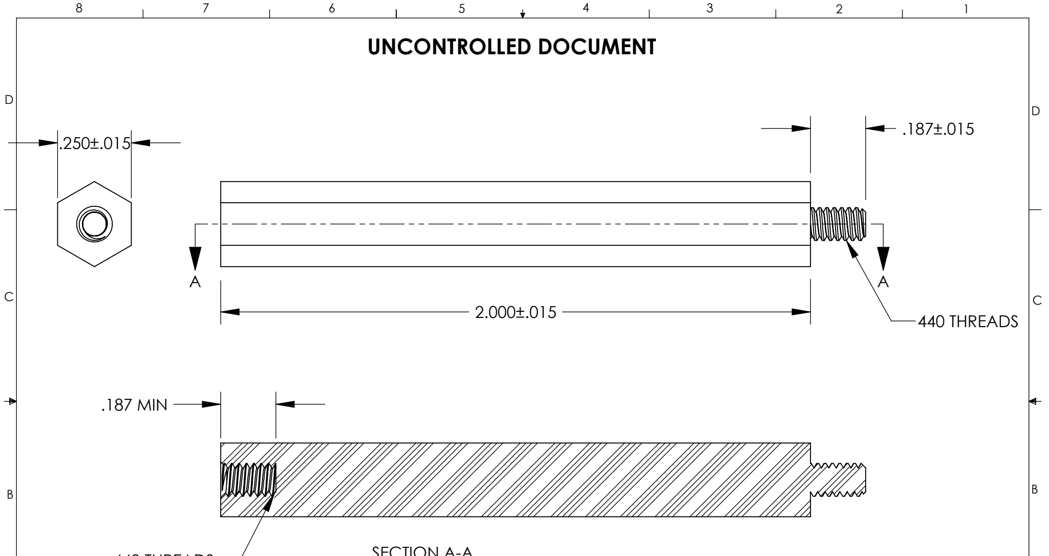
SECTION A-A 440 THREADS
