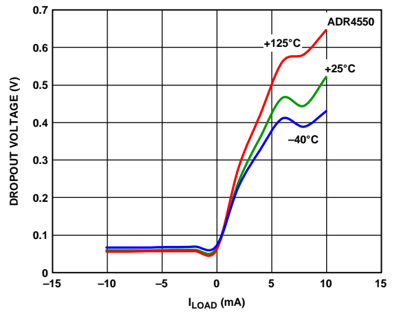
Figure 90. ADR4550 Dropout Voltage vs. Load Current
