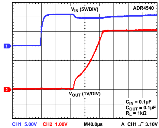
Figure 68. ADR4540 Output Voltage Start-Up Response
