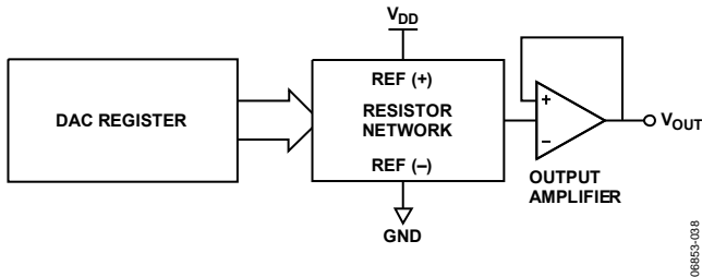
Figure 39. DAC Architecture
