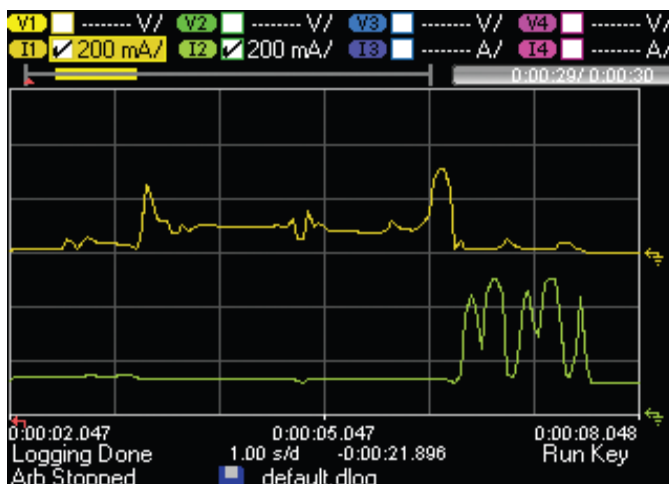
Figure 6. In Data Logger View, you can log data on multiple traces. Here, the current flowing out of output 1 and output 2 are captured over 30 seconds.
