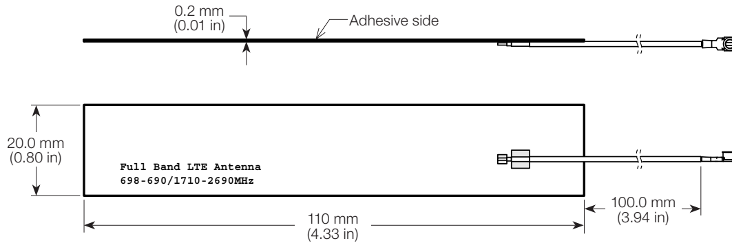
Figure 6. ANT-LPL-FPC-100 Dimensions
