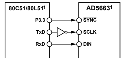
ADDITIONAL PINS OMITTED FOR CLARITY.
