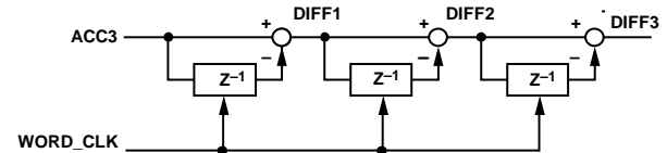
Figure 26. Differentiator
