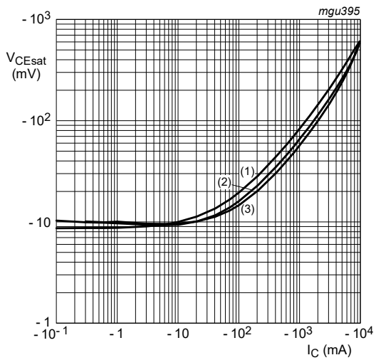
I_C/I_B = 20 (1) T_{amb} = 150\text{ }^{\circ}C (2) T_{amb} = 25\text{ }^{\circ}C (3) T_{amb} = -55\text{ }^{\circ}C
