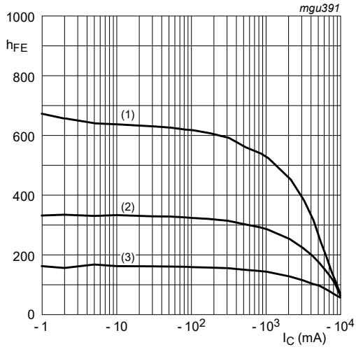
V_{CE} = -2 V (1) T_{amb} = 150\text{ }^{\circ}C (2) T_{amb} = 25\text{ }^{\circ}C (3) T_{amb} = -55\text{ }^{\circ}C
