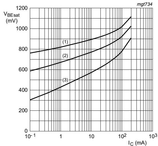
Fig. 13. Group C: Base-emitter voltage as a function of collector current; typical values
