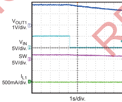
Enable down I_{OUT1} = I_{OUT2} = 0A
