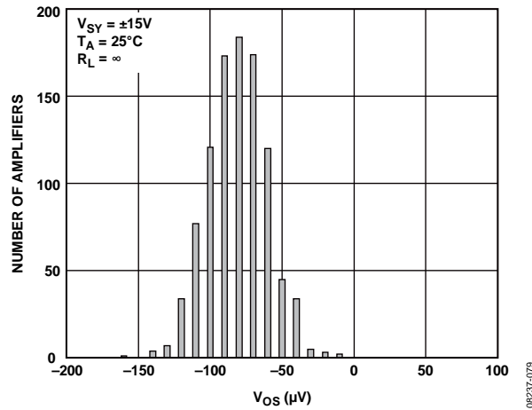
Figure 75. Input Offset Voltage ( V_{OS} ) Distribution, LFCSP
