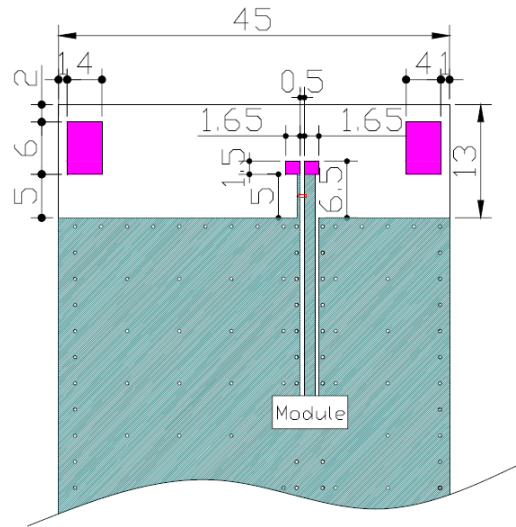
Figure 16. Layout dimensions of the PA700J Antenna.
