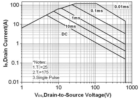
Safe Operating Area T_c=25^\circ C, V_{ge}=15V
