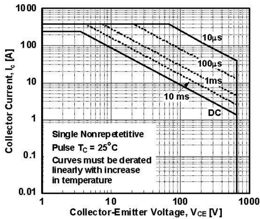
SOA Characteristics
