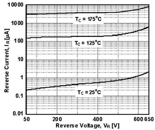
Reverse Current
