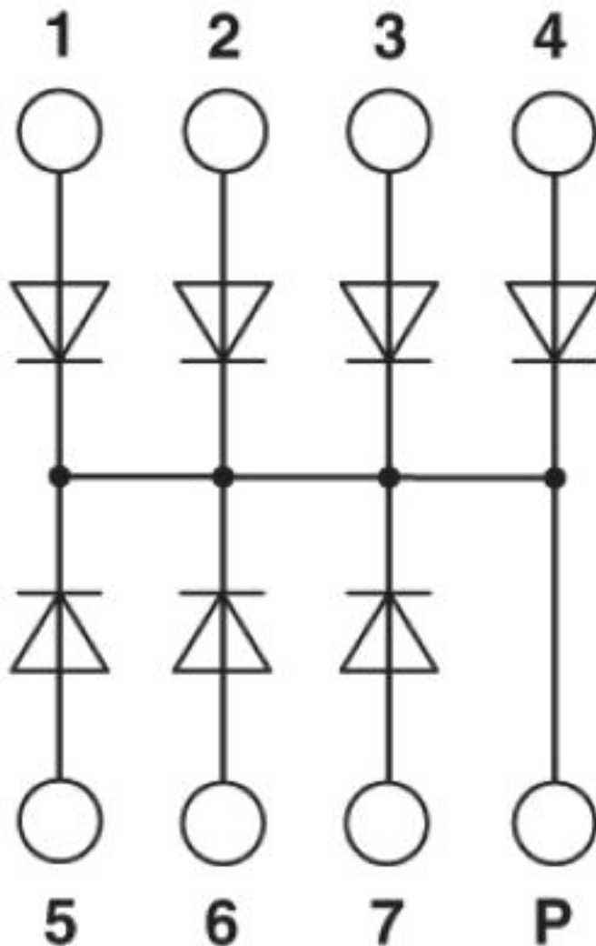
Circuit diagram
